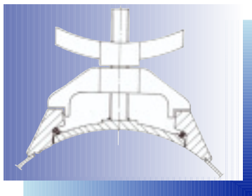
Diamant-Putzdeckel/diamant caps
